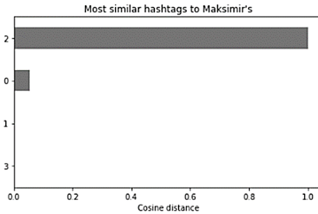
Figure 3.6 Cosine distance
