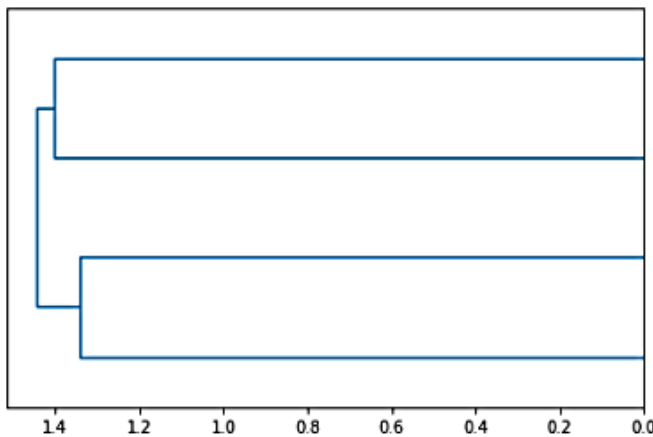
Figure 3.7 Hierarchical clustering
