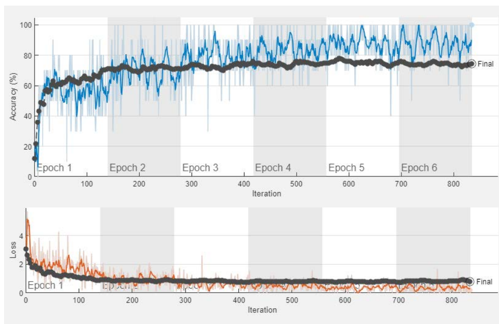
Figure 3.9 Training progress
